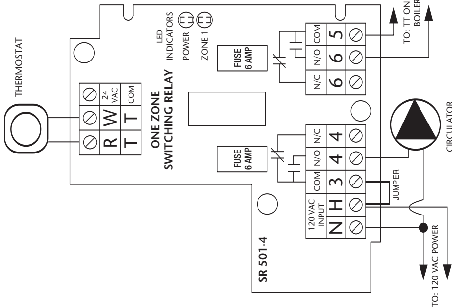
TYPICAL WIRING (COLD START)
