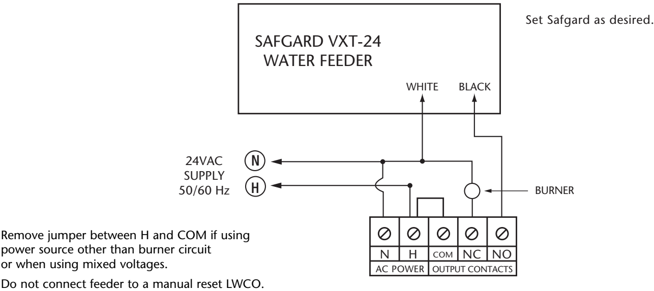
24 VAC LWCO Using Burner Circuit Power Source
