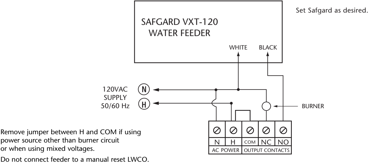
120 VAC LWCO Using Burner Circuit Power Source
