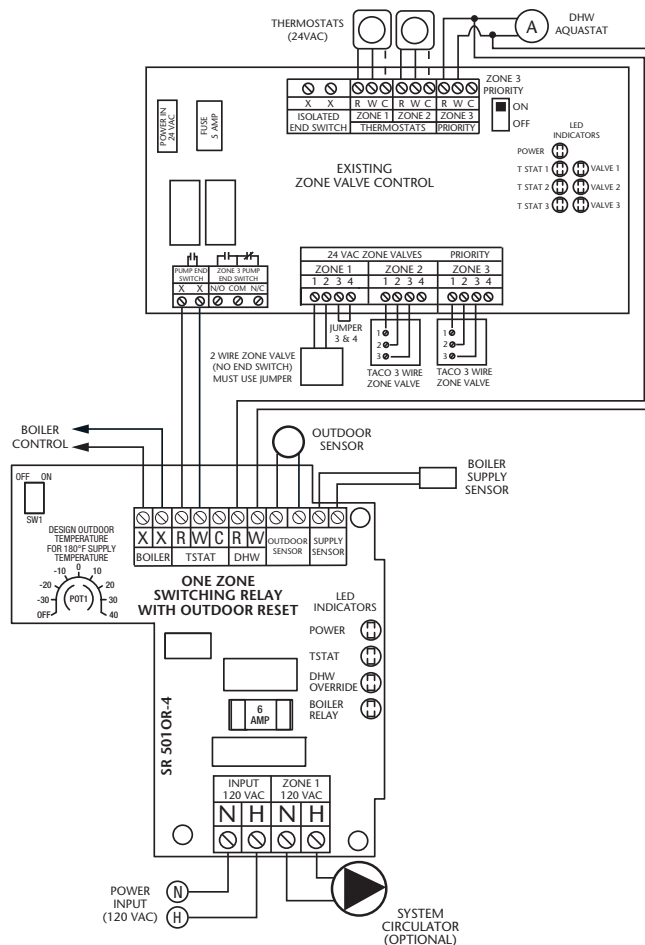
MULTI-ZONE INSTALLATION WITH ZONE CONTROL, WITH INDIRECT DHW
